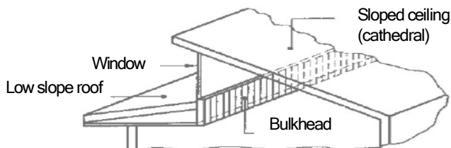
(e) Saw-tooth roof construction
