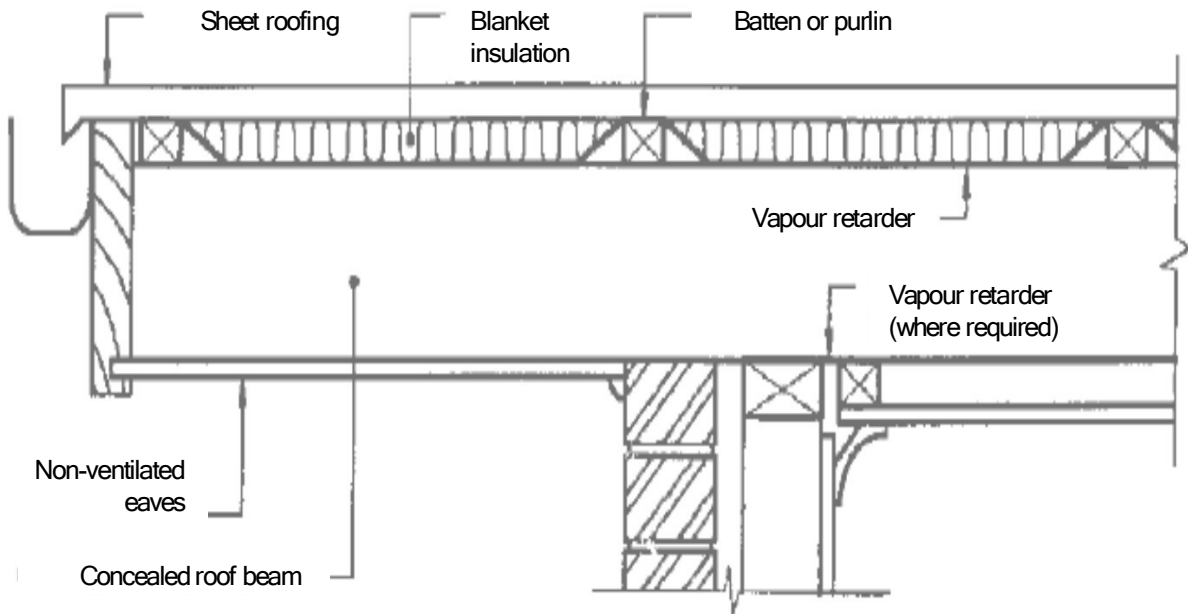
Illustration 8: Blanket insulation in contact with roof sheeting.
