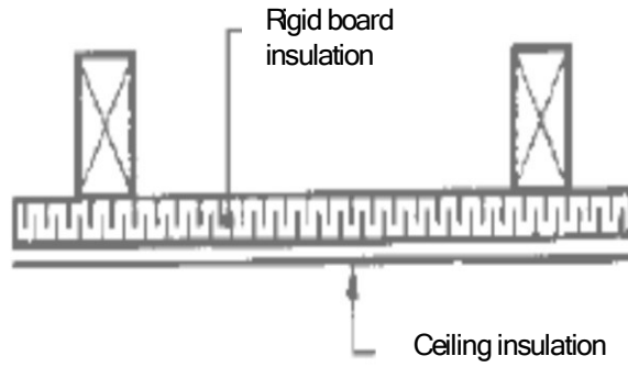
Illustration 7: Rigid board installed between ceiling joists and lining
