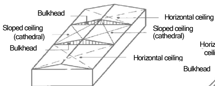
(c) Terrace construction
