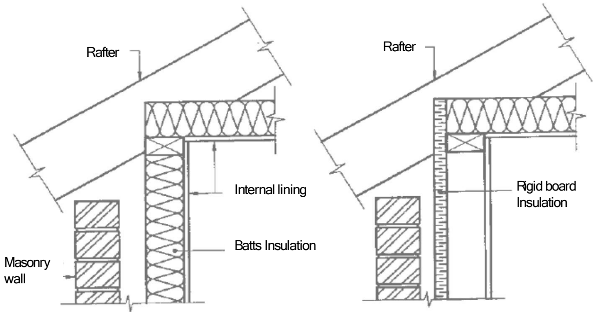
Illustration 1: Placement of thermal insulation to eliminate thermal bridging.
