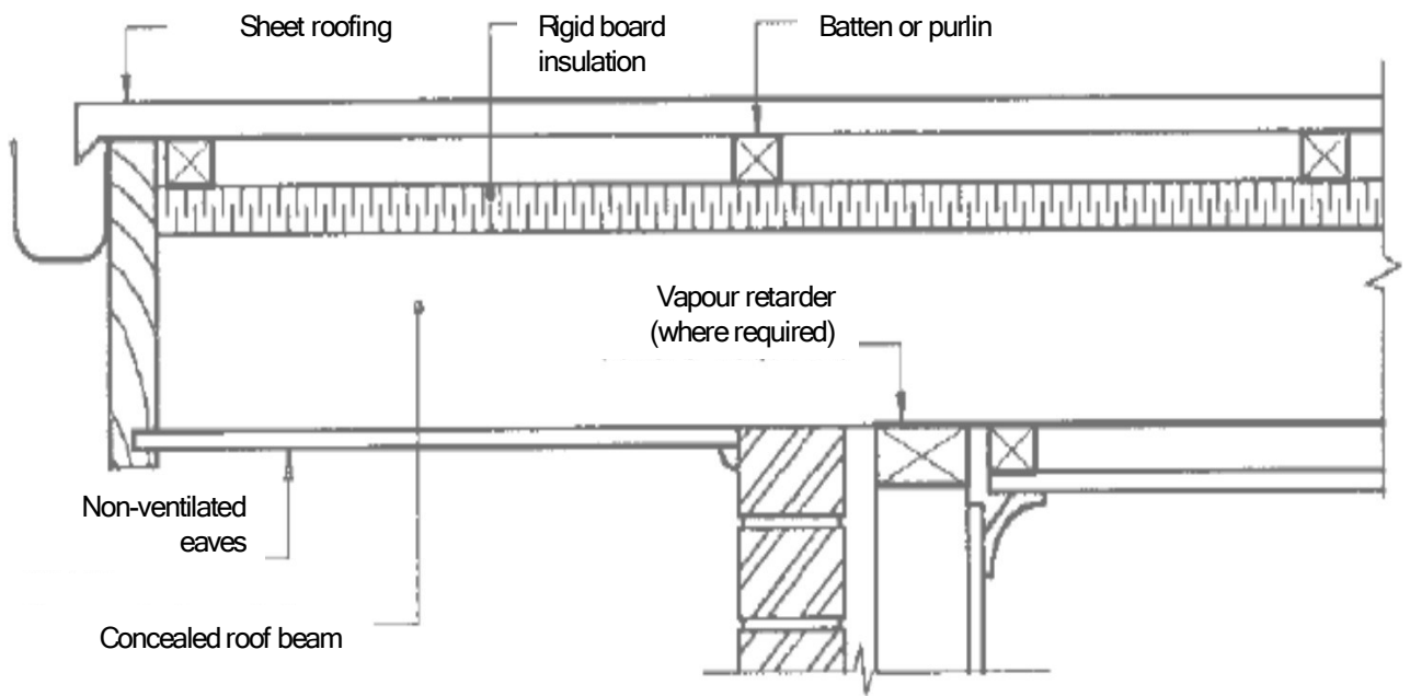
Illustration 10: Rigid board insulation beneath roofing battens.
