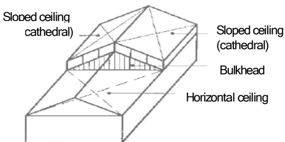
(b) Split level construction
