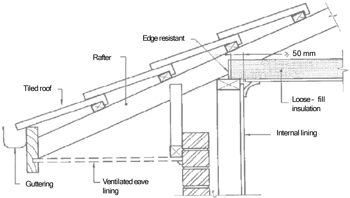
Illustration 2: Edge restraint for loose-fill insulation where eaves are ventilated (CFI)
