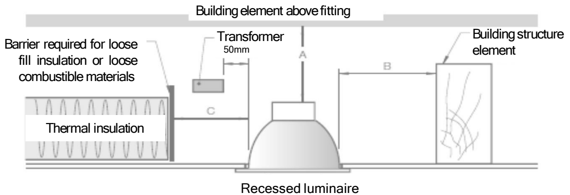
Illustration 5: Alternative treatments for drop ceilings or cavities below ceiling line.
